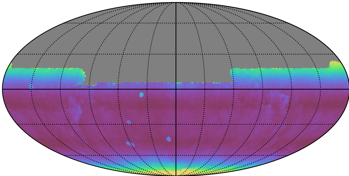
noroll_mjdp180_v3.4_10yrs All sky y band: Median airmass
