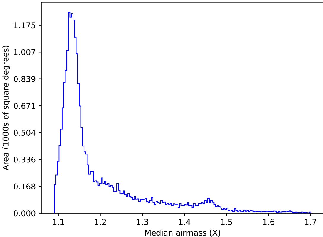
noroll_mjdp180_v3.4_10yrs All sky y band: Median airmass
