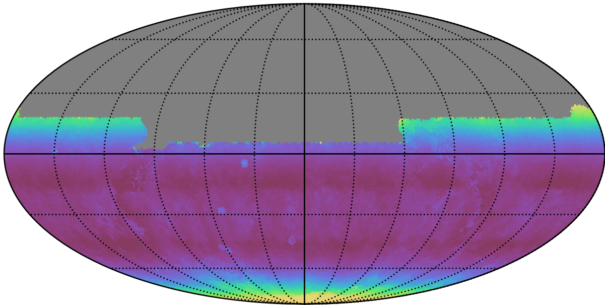
noroll_mjdp180_v3.4_10yrs All sky u band: Median airmass
