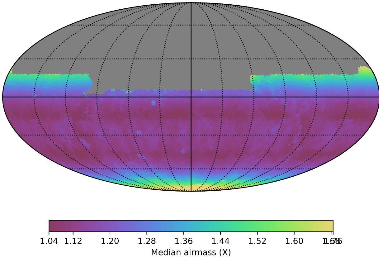
noroll_mjdp180_v3.4_10yrs All sky u band: Median airmass
