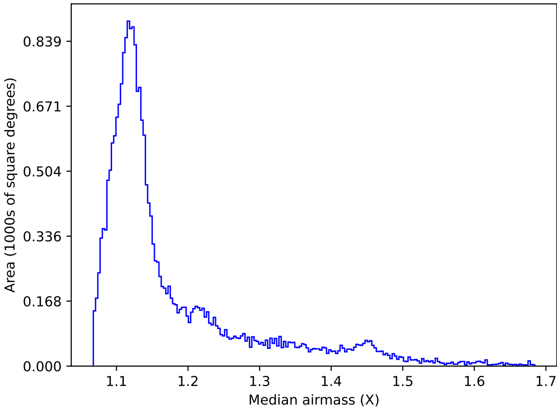
noroll_mjdp180_v3.4_10yrs All sky u band: Median airmass
