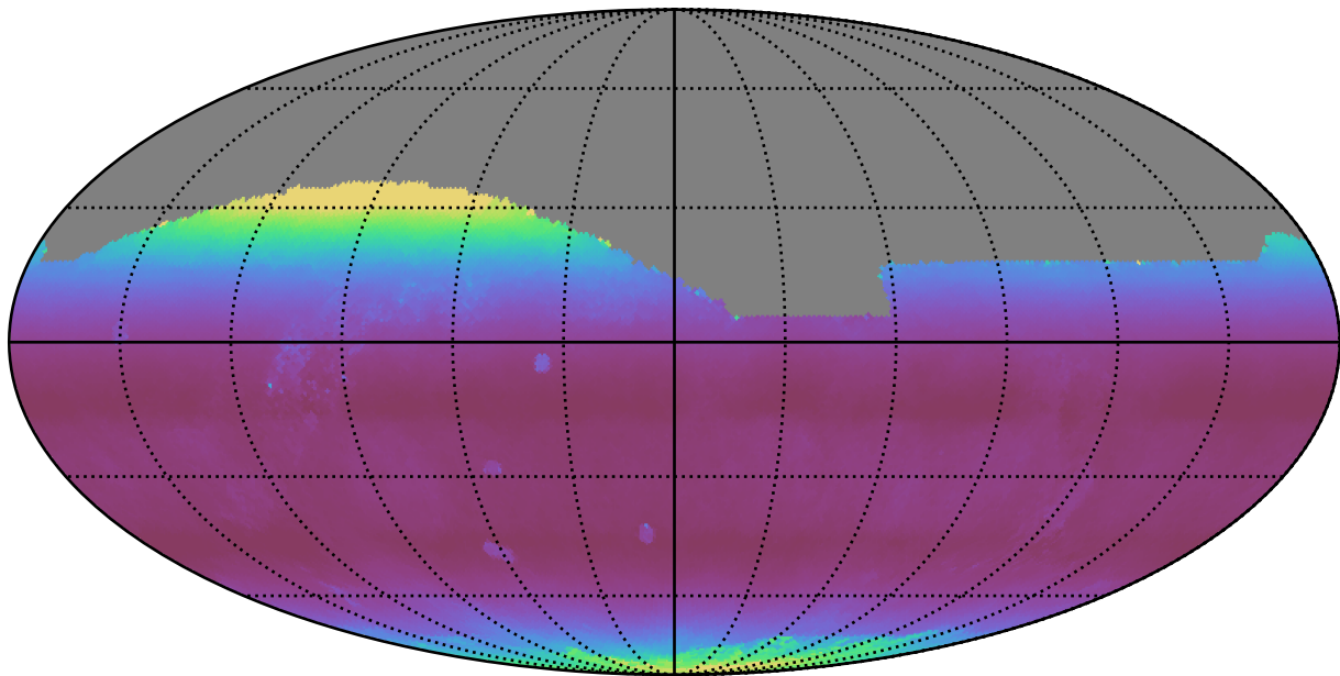
noroll_mjdp180_v3.4_10yrs All sky r band: Median airmass
