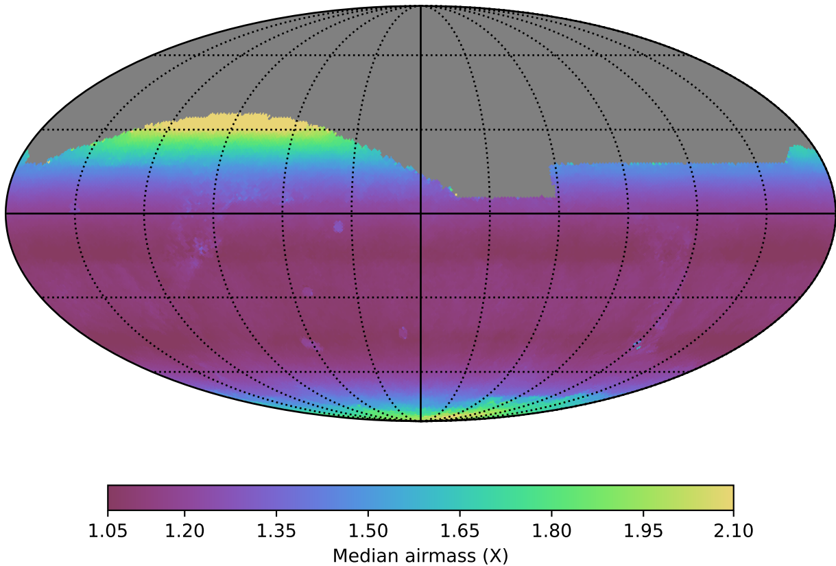
noroll_mjdp180_v3.4_10yrs All sky i band: Median airmass
