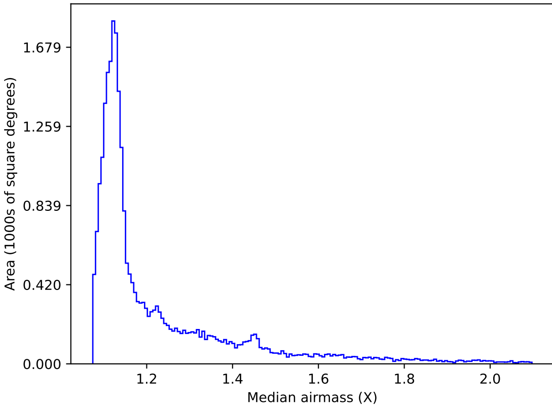
noroll_mjdp180_v3.4_10yrs All sky i band: Median airmass
