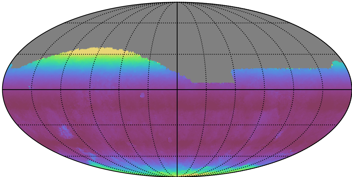
noroll_mjdp180_v3.4_10yrs All sky g band: Median airmass
