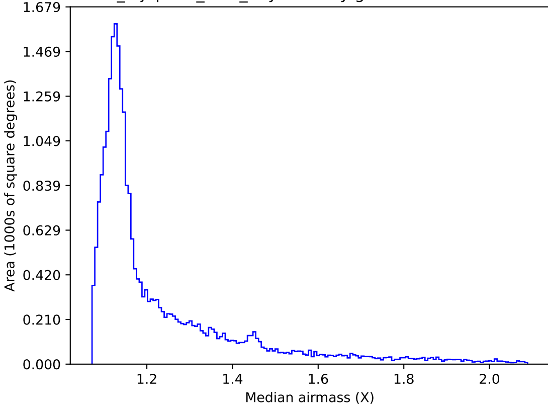
noroll_mjdp180_v3.4_10yrs All sky g band: Median airmass
