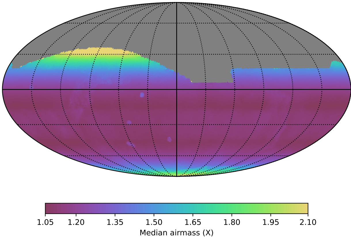
noroll_mjdp180_v3.4_10yrs All sky all bands: Median airmass
