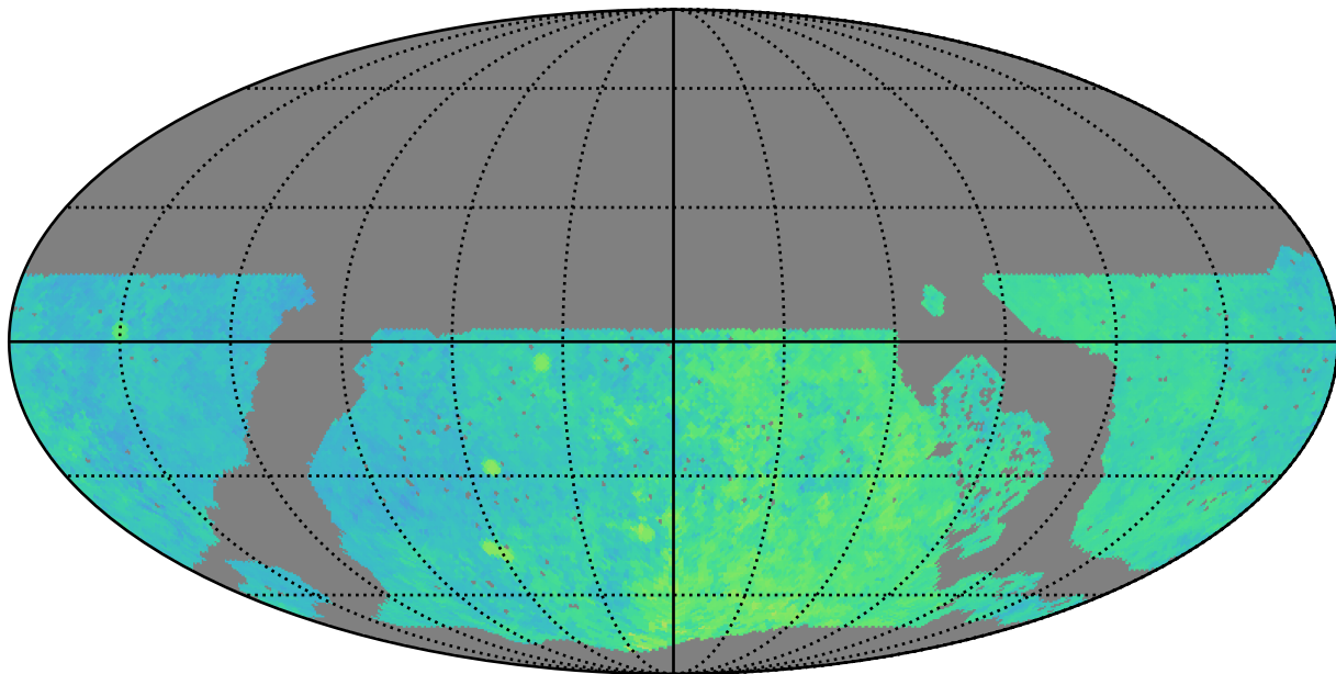
noroll_mjdp180_v3.4_10yrs WFD z band: Median Season Length
