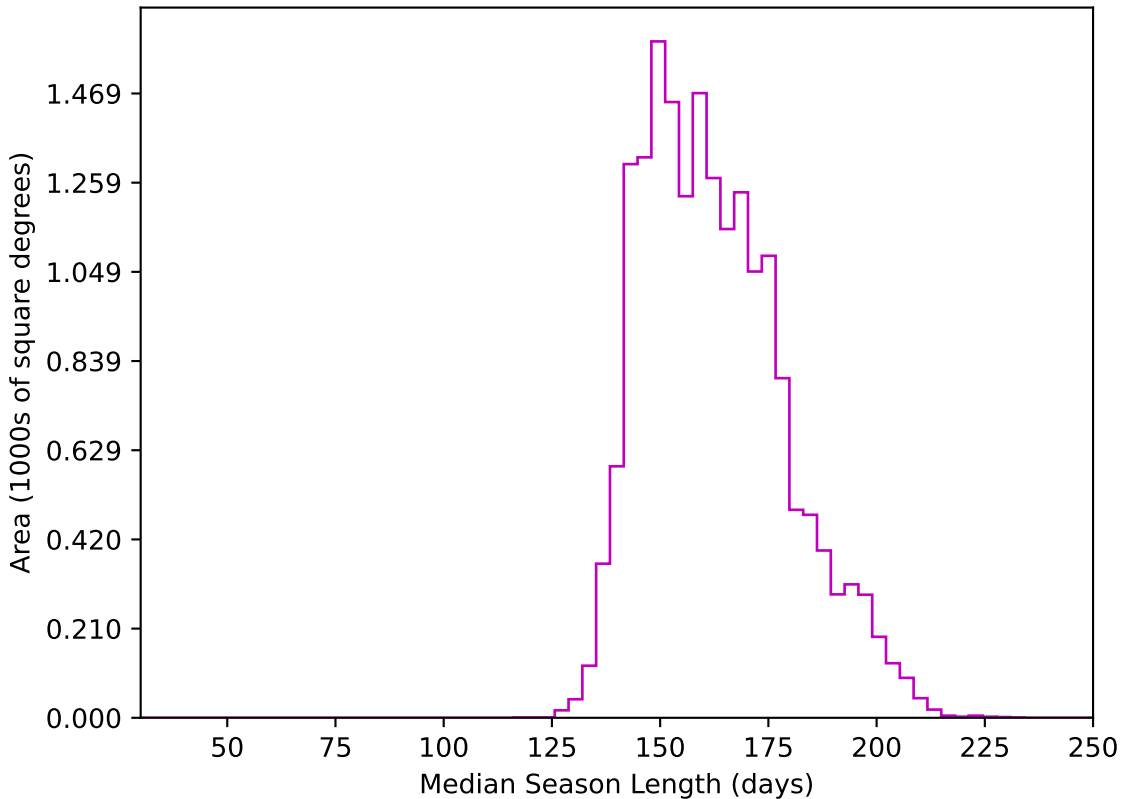
noroll_mjdp180_v3.4_10yrs WFD z band: Median Season Length
