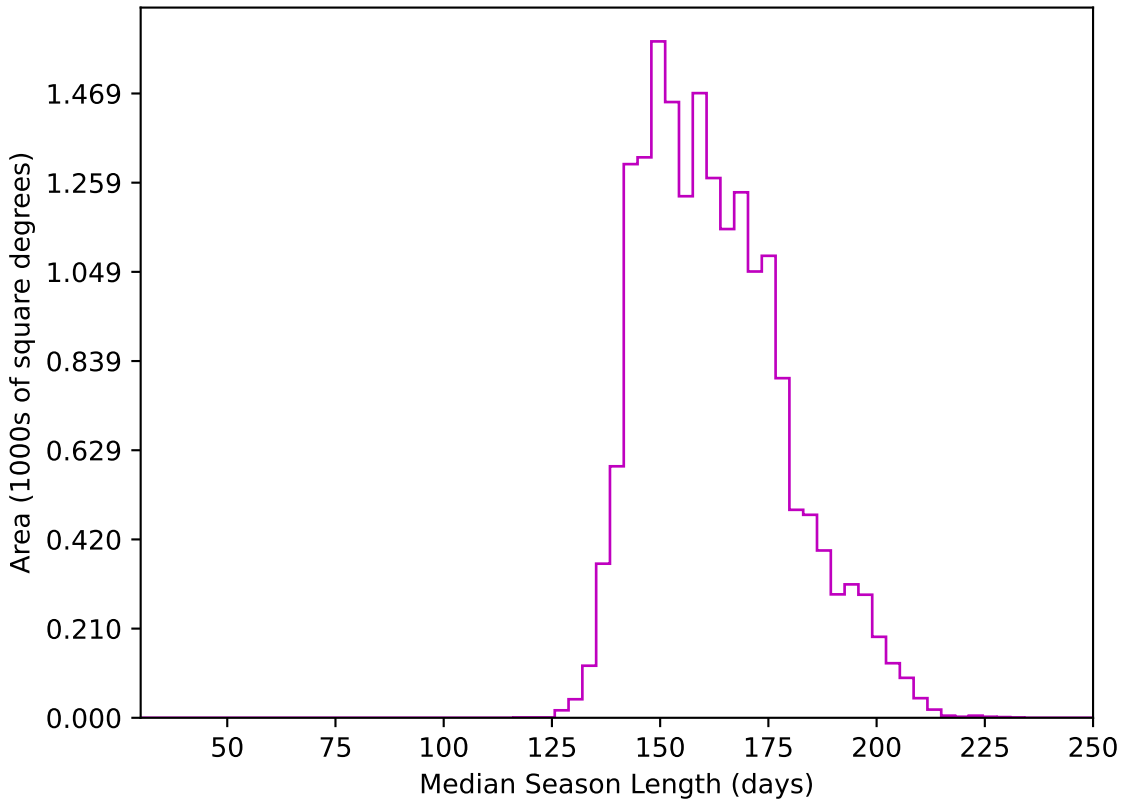
noroll_mjdp180_v3.4_10yrs WFD z band: Median Season Length
