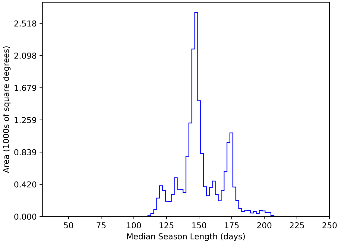
noroll_mjdp180_v3.4_10yrs WFD y band: Median Season Length
