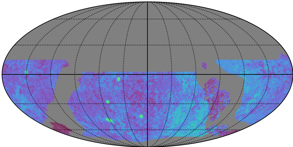
noroll_mjdp180_v3.4_10yrs WFD u band: Median Season Length
