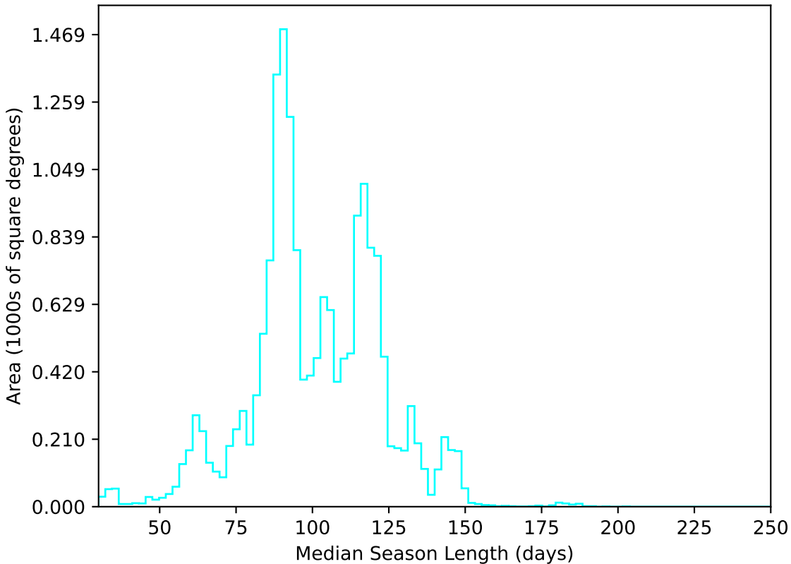
noroll_mjdp180_v3.4_10yrs WFD u band: Median Season Length
