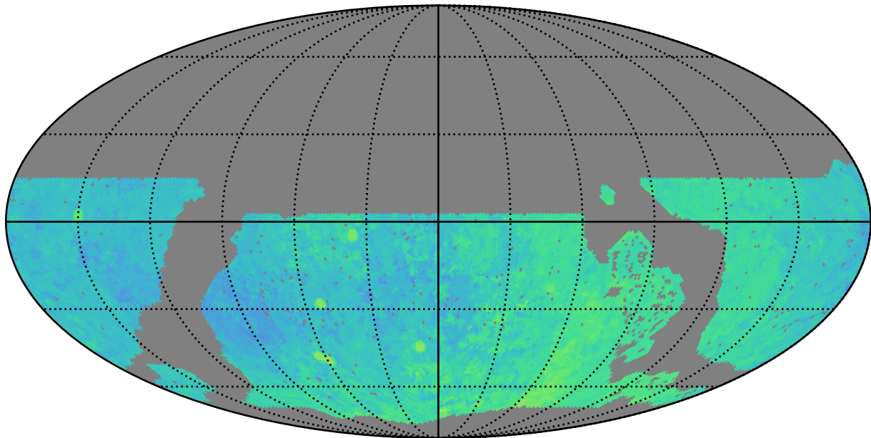
noroll_mjdp180_v3.4_10yrs WFD r band: Median Season Length
