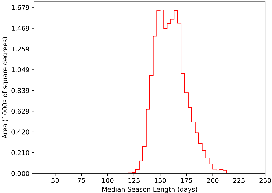
noroll_mjdp180_v3.4_10yrs WFD i band: Median Season Length
