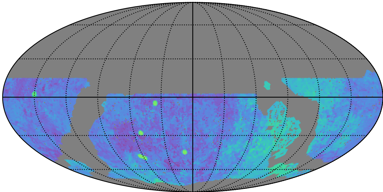
noroll_mjdp180_v3.4_10yrs WFD g band: Median Season Length
