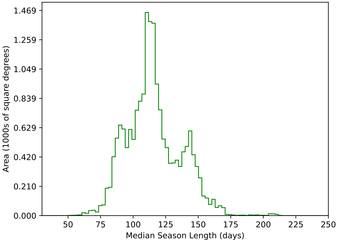
noroll_mjdp180_v3.4_10yrs WFD g band: Median Season Length
