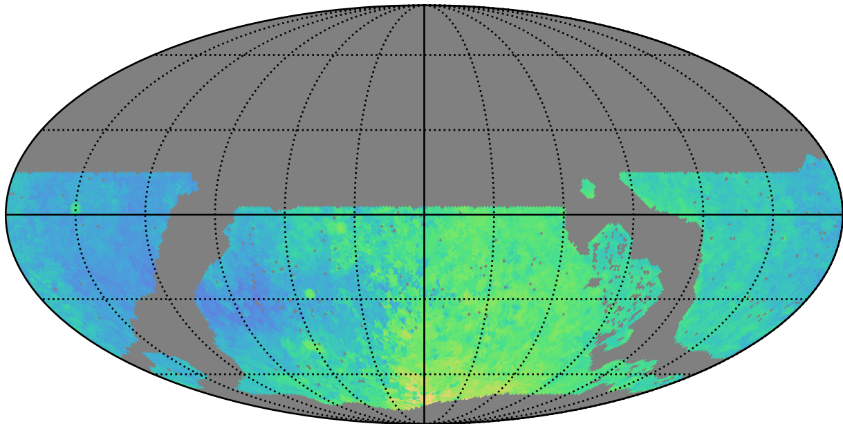
noroll_mjdp180_v3.4_10yrs WFD all bands: Median Season Length
