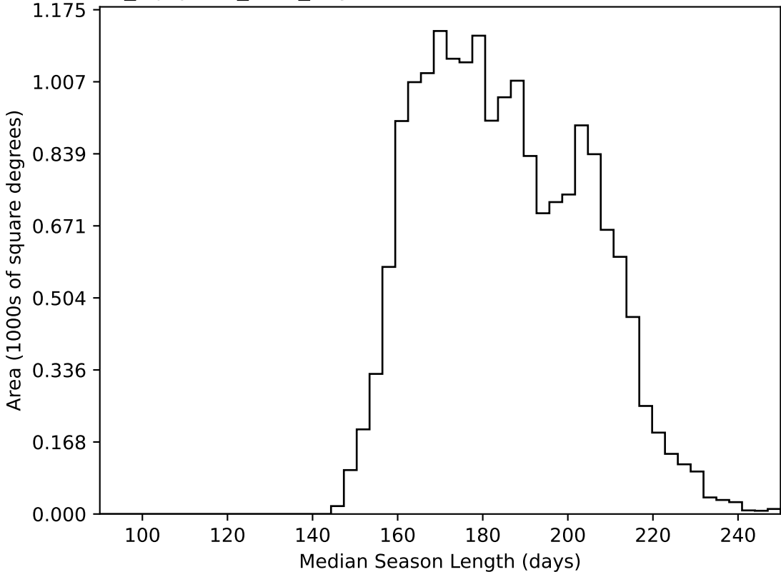
noroll_mjdp180_v3.4_10yrs WFD all bands: Median Season Length
