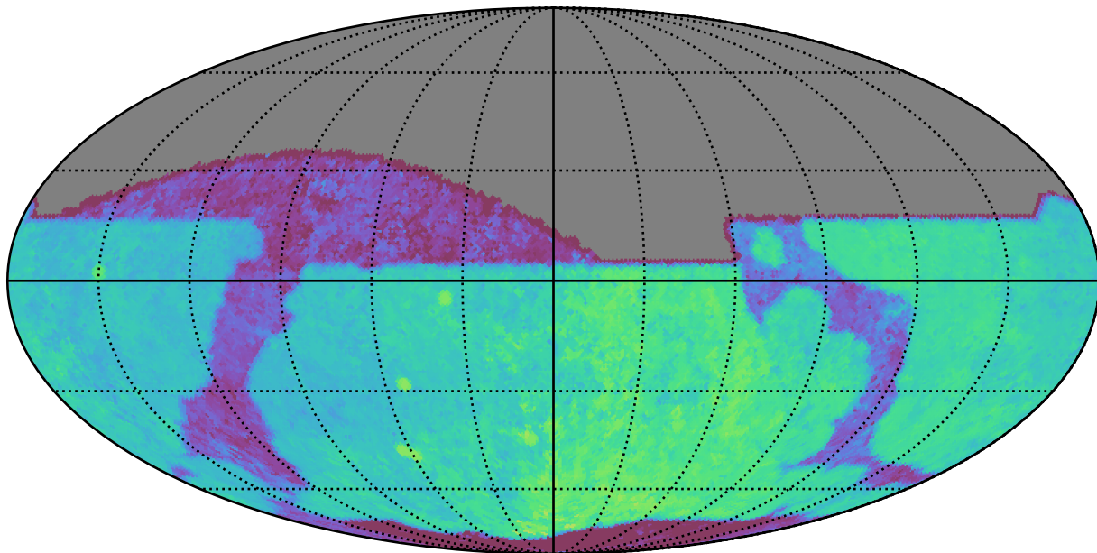
noroll_mjdp180_v3.4_10yrs All sky z band: Median Season Length
