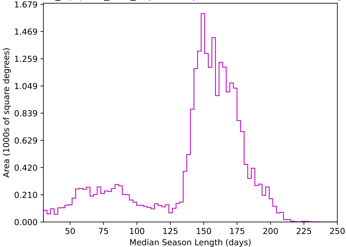
noroll_mjdp180_v3.4_10yrs All sky z band: Median Season Length
