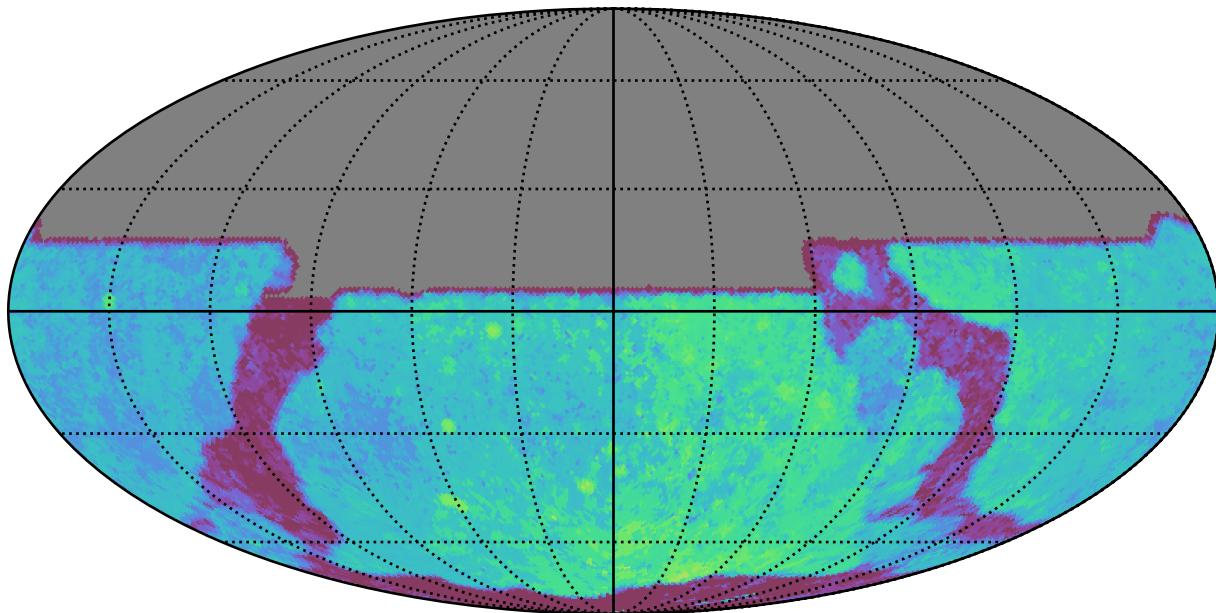
noroll_mjdp180_v3.4_10yrs All sky y band: Median Season Length
