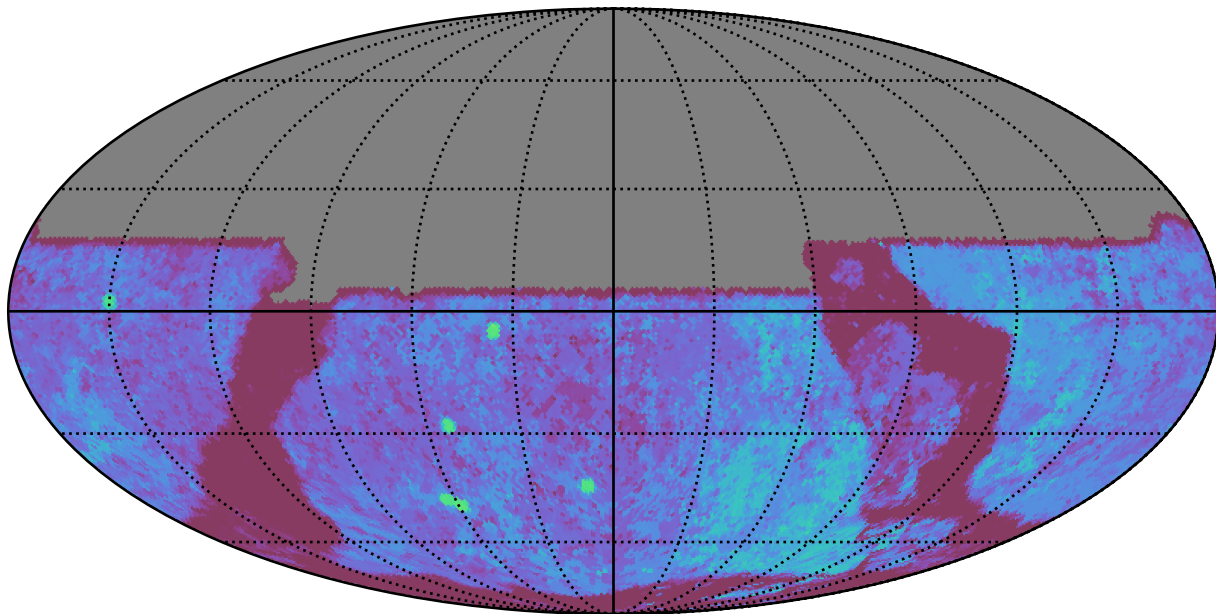
noroll_mjdp180_v3.4_10yrs All sky u band: Median Season Length
