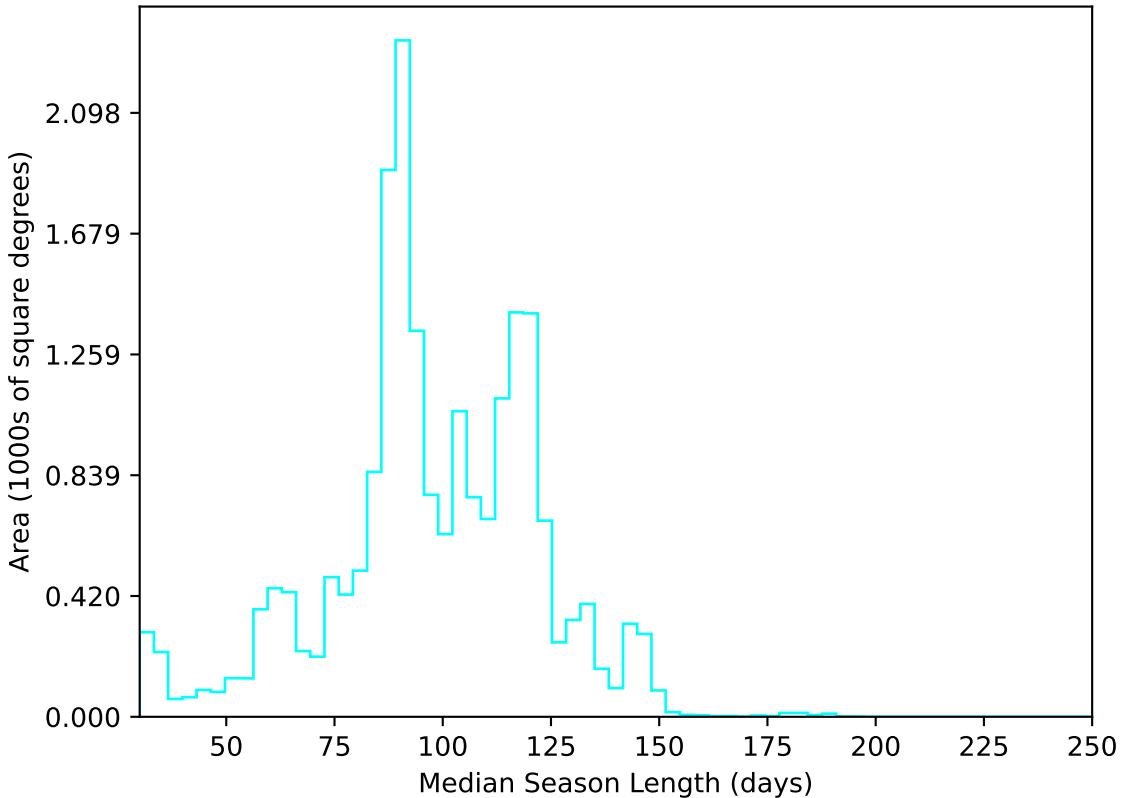
noroll_mjdp180_v3.4_10yrs All sky u band: Median Season Length
