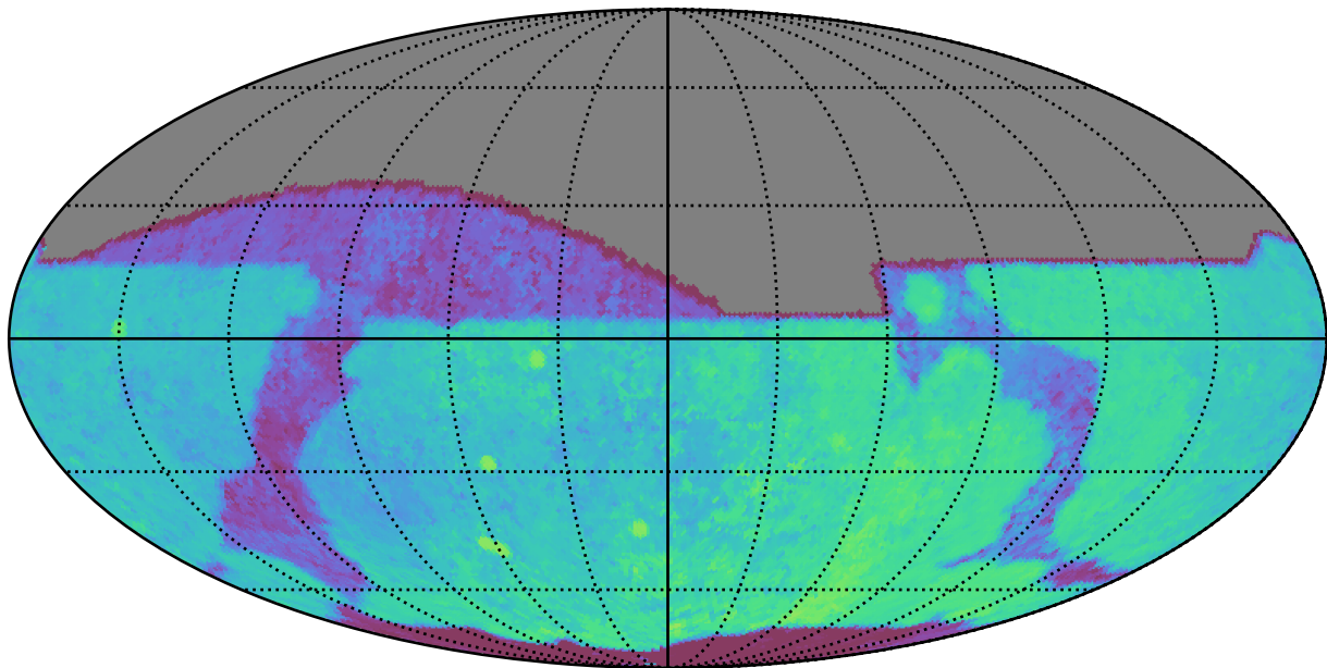
noroll_mjdp180_v3.4_10yrs All sky r band: Median Season Length
