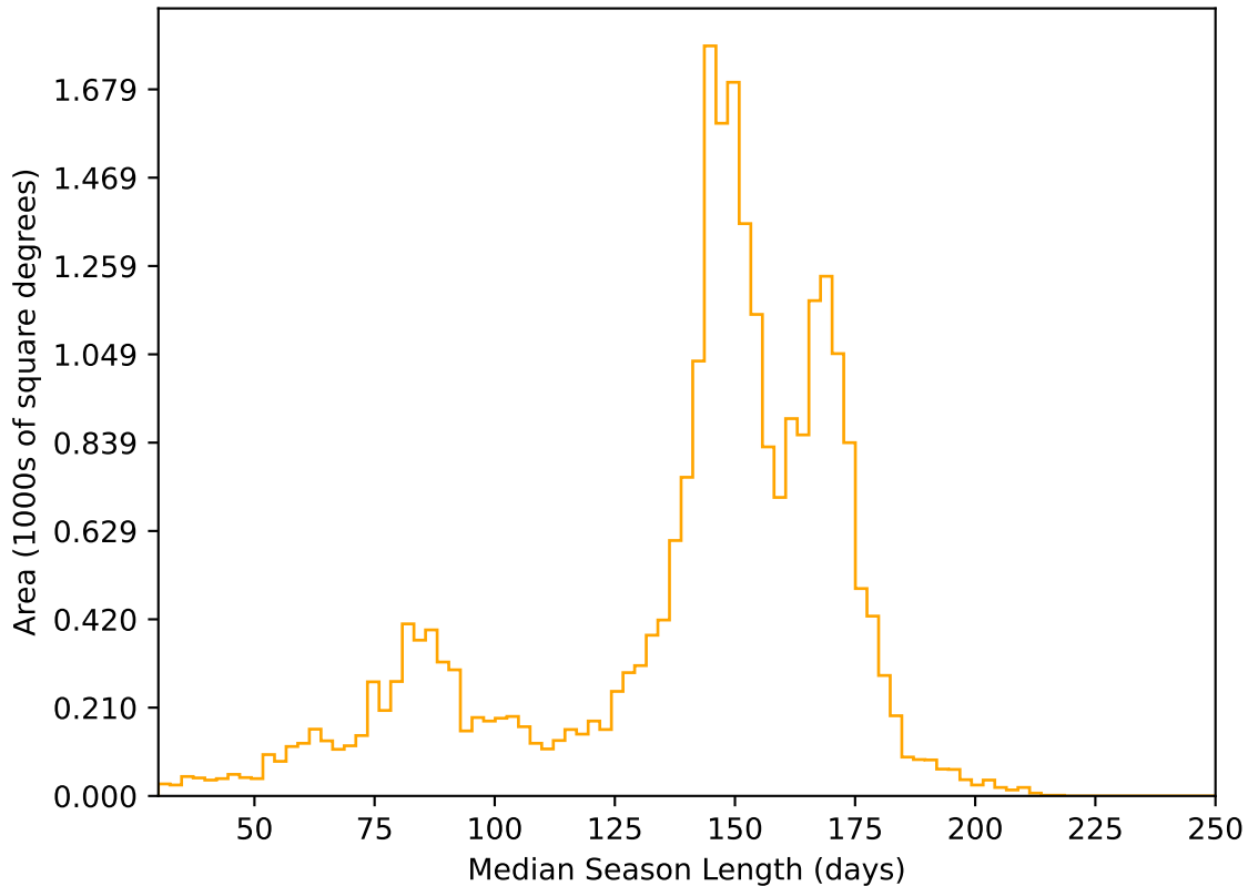
noroll_mjdp180_v3.4_10yrs All sky r band: Median Season Length
