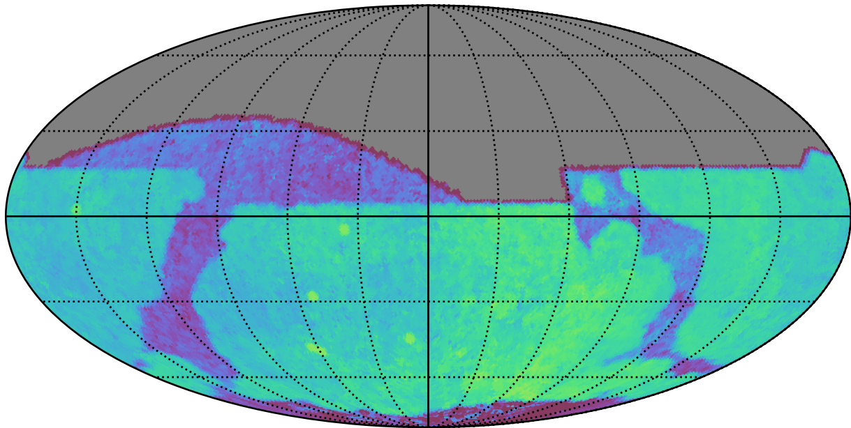
noroll_mjdp180_v3.4_10yrs All sky i band: Median Season Length
