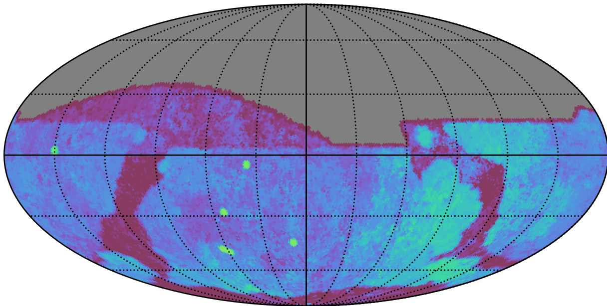
noroll_mjdp180_v3.4_10yrs All sky g band: Median Season Length
