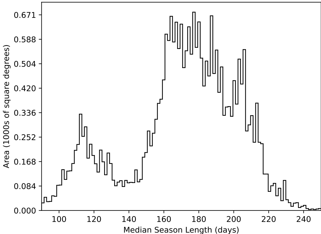
noroll_mjdp180_v3.4_10yrs All sky all bands: Median Season Length
