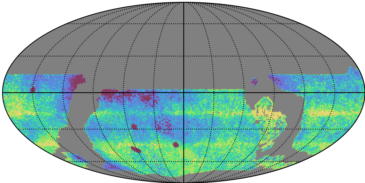
noroll_mjdp180_v3.4_10yrs WFD: Median Intra-Night Gap
