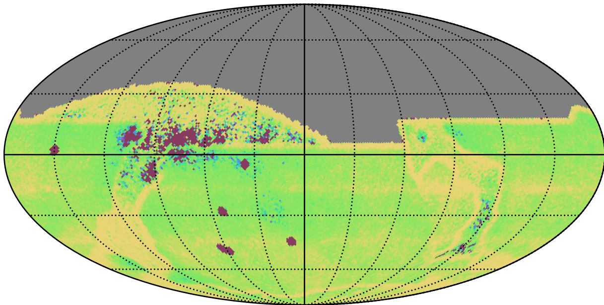
noroll_mjdp180_v3.4_10yrs All sky: Median Intra-Night Gap
