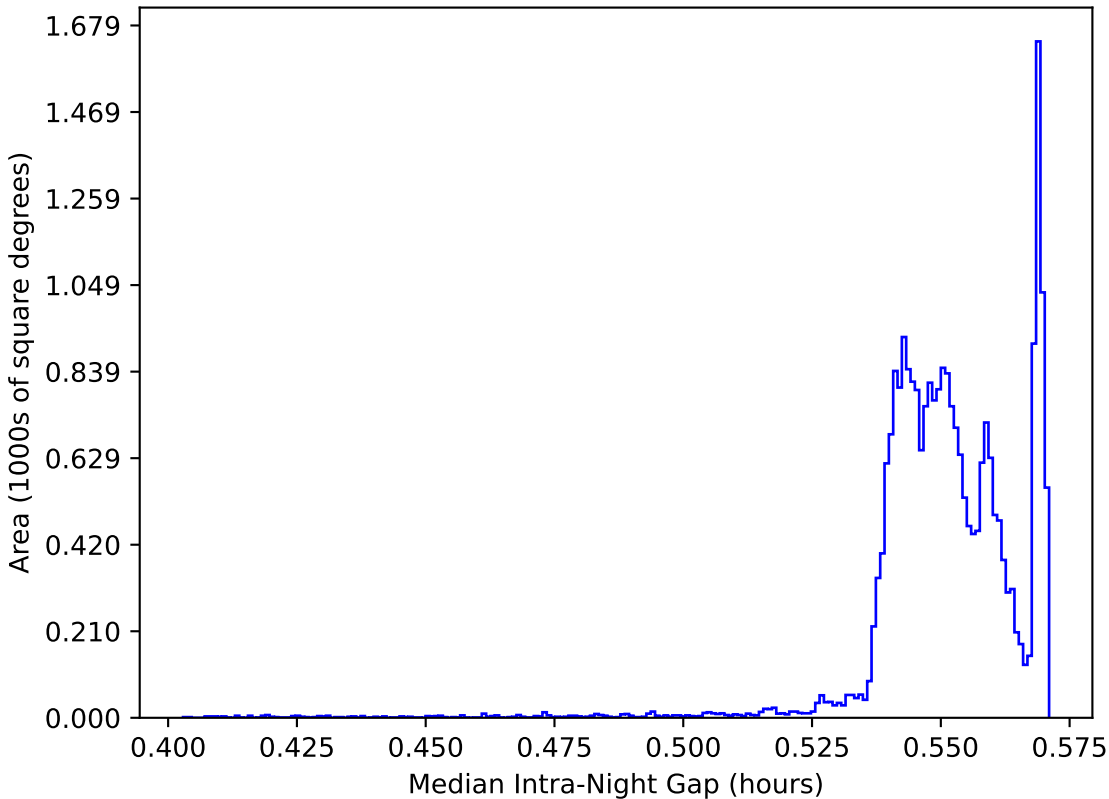
noroll_mjdp180_v3.4_10yrs All sky: Median Intra-Night Gap
