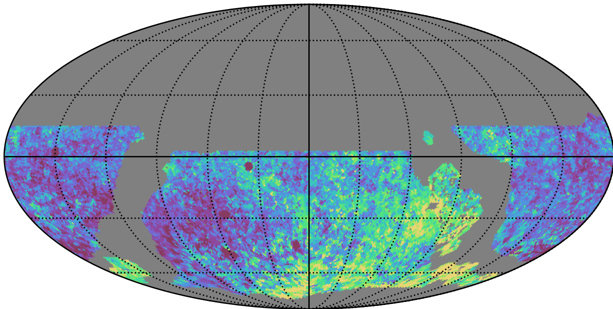
noroll_mjdp180_v3.4_10yrs WFD z band: Median Inter-Night Gap
