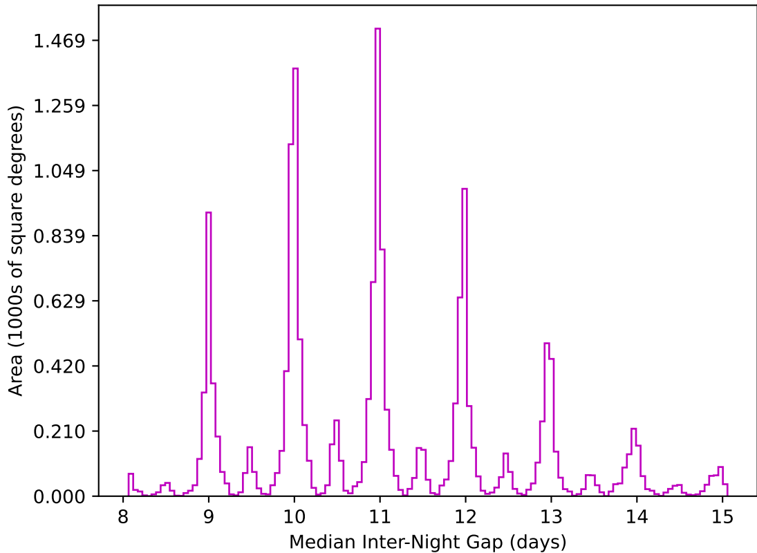
noroll_mjdp180_v3.4_10yrs WFD z band: Median Inter-Night Gap
