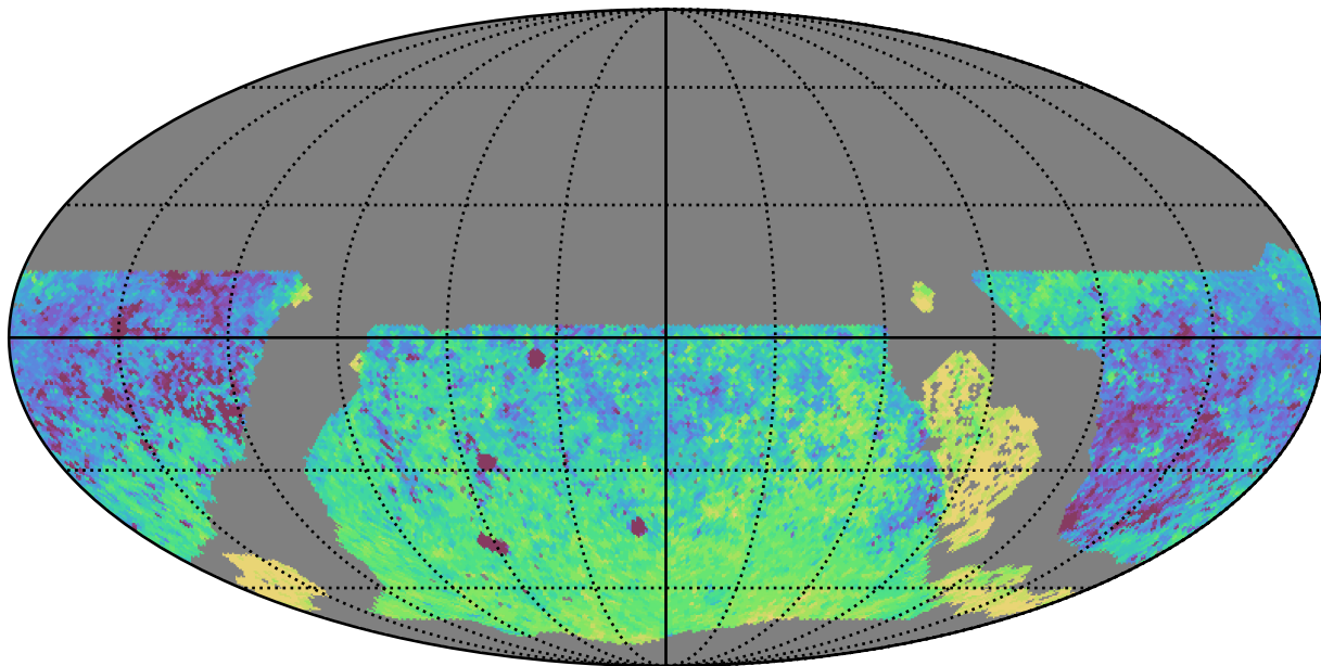
noroll_mjdp180_v3.4_10yrs WFD y band: Median Inter-Night Gap
