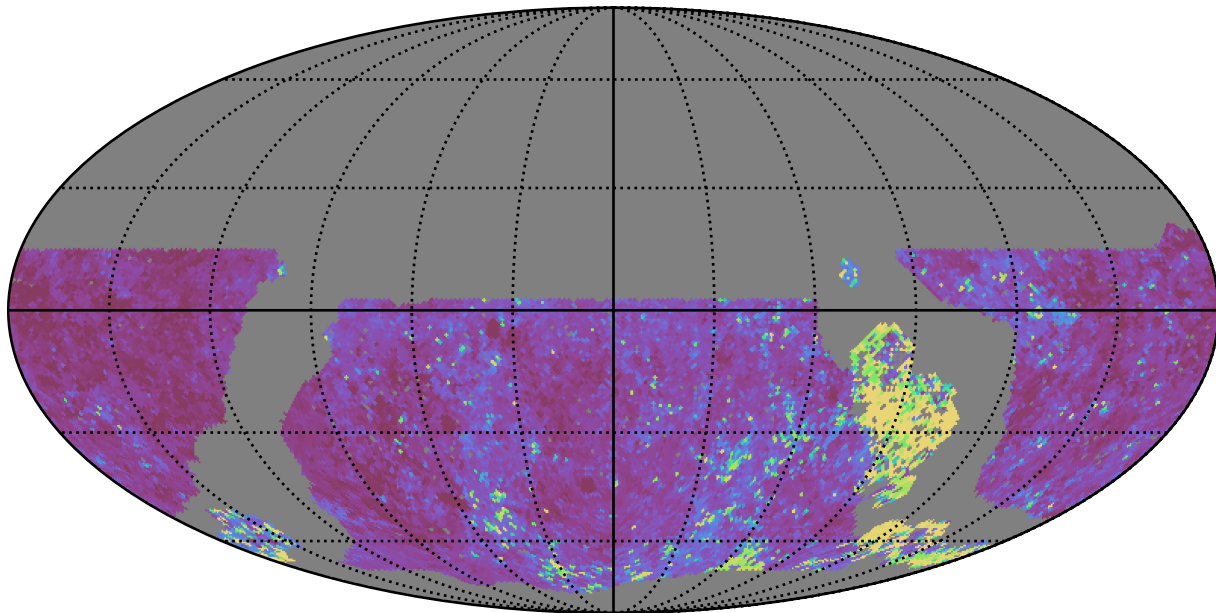
noroll_mjdp180_v3.4_10yrs WFD u band: Median Inter-Night Gap
