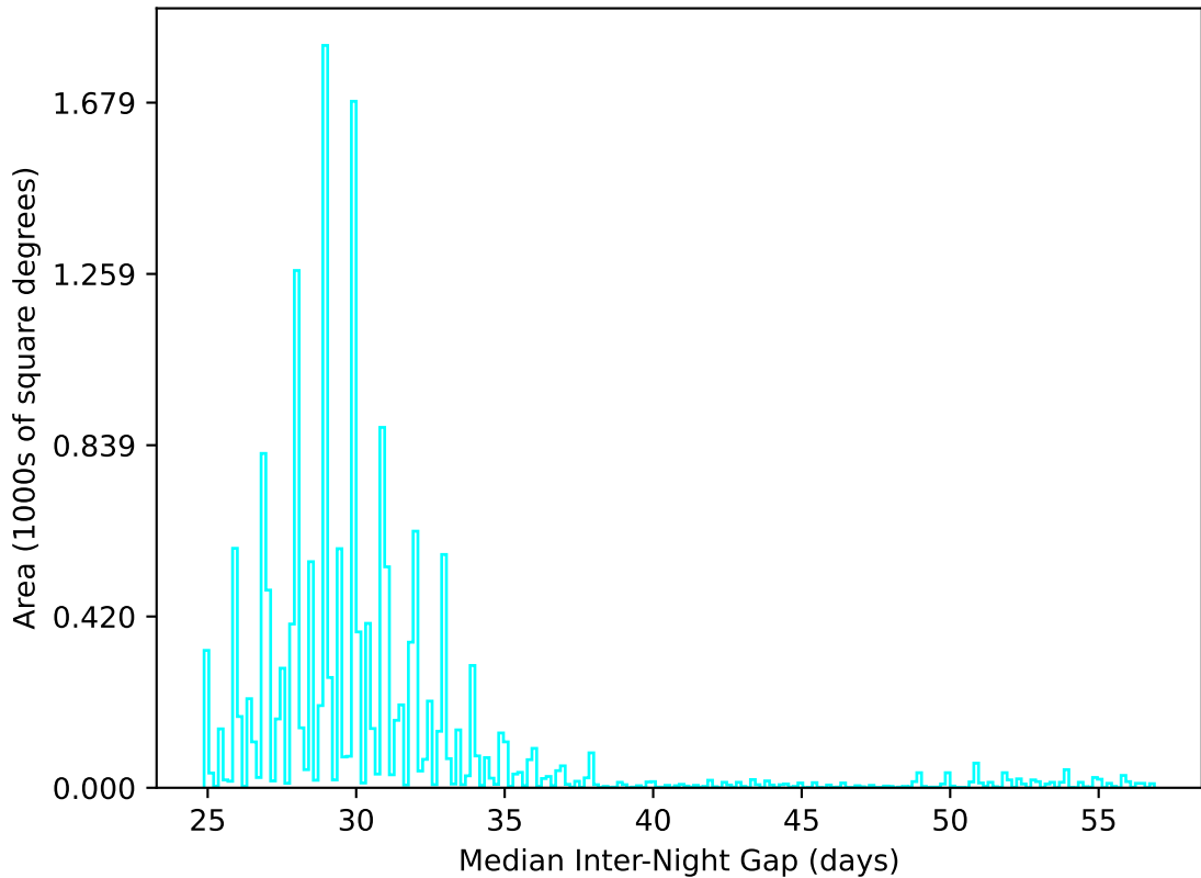
noroll_mjdp180_v3.4_10yrs WFD u band: Median Inter-Night Gap
