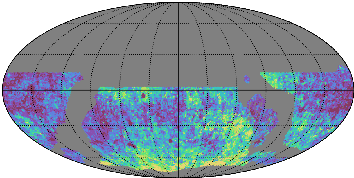
noroll_mjdp180_v3.4_10yrs WFD r band: Median Inter-Night Gap
