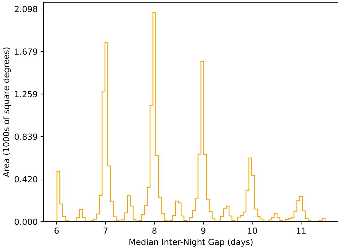
noroll_mjdp180_v3.4_10yrs WFD r band: Median Inter-Night Gap
