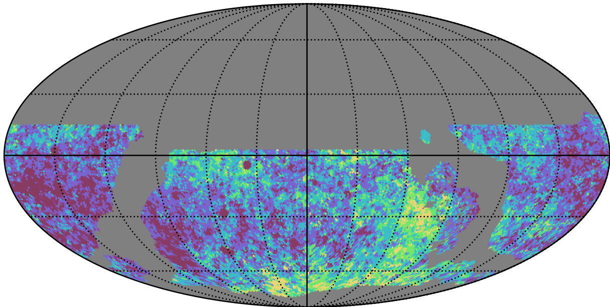
noroll_mjdp180_v3.4_10yrs WFD i band: Median Inter-Night Gap
