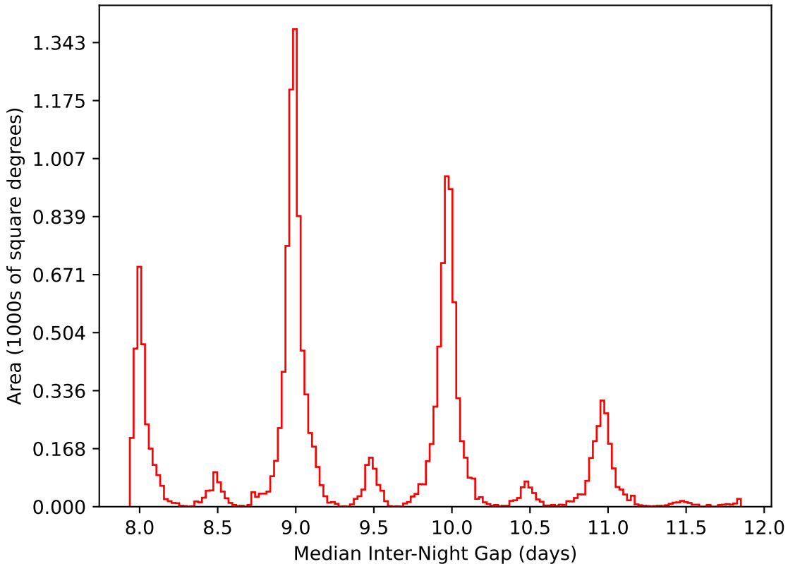
noroll_mjdp180_v3.4_10yrs WFD i band: Median Inter-Night Gap
