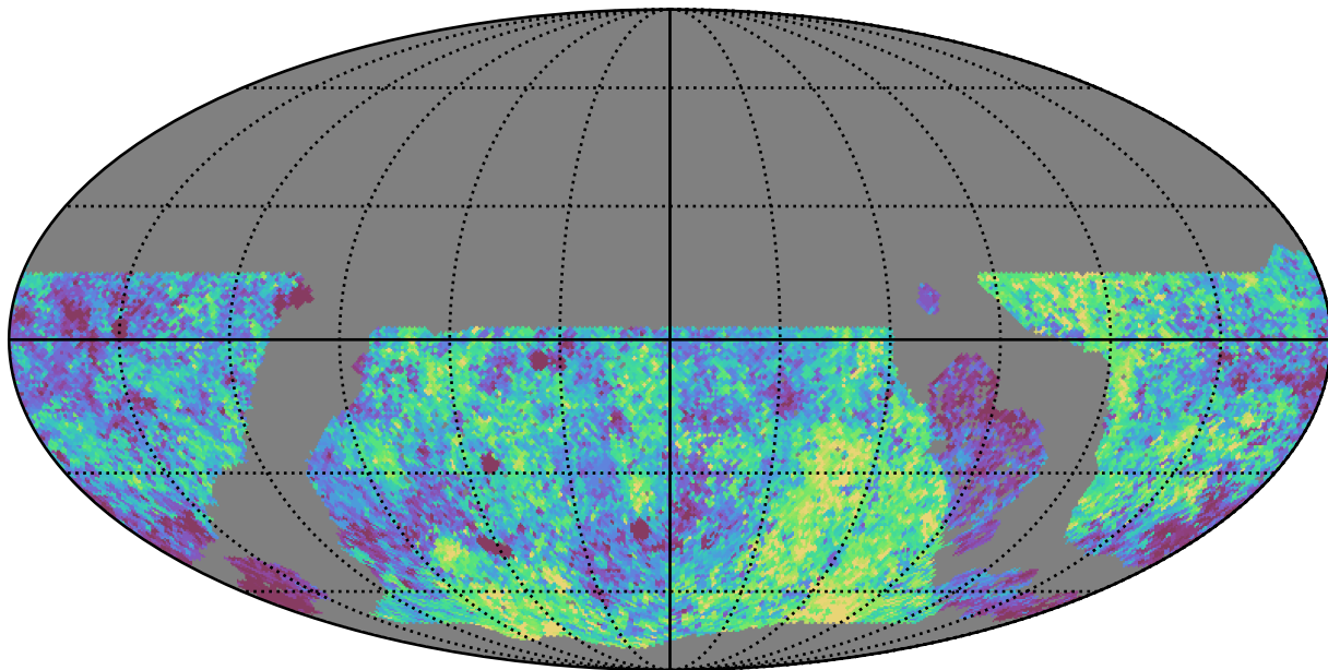
noroll_mjdp180_v3.4_10yrs WFD g band: Median Inter-Night Gap
