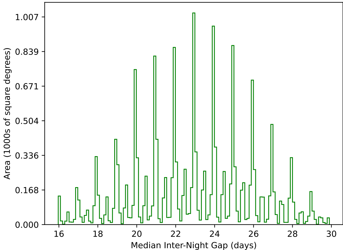
noroll_mjdp180_v3.4_10yrs WFD g band: Median Inter-Night Gap
