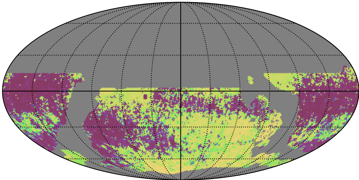
noroll_mjdp180_v3.4_10yrs WFD all bands: Median Inter-Night Gap
