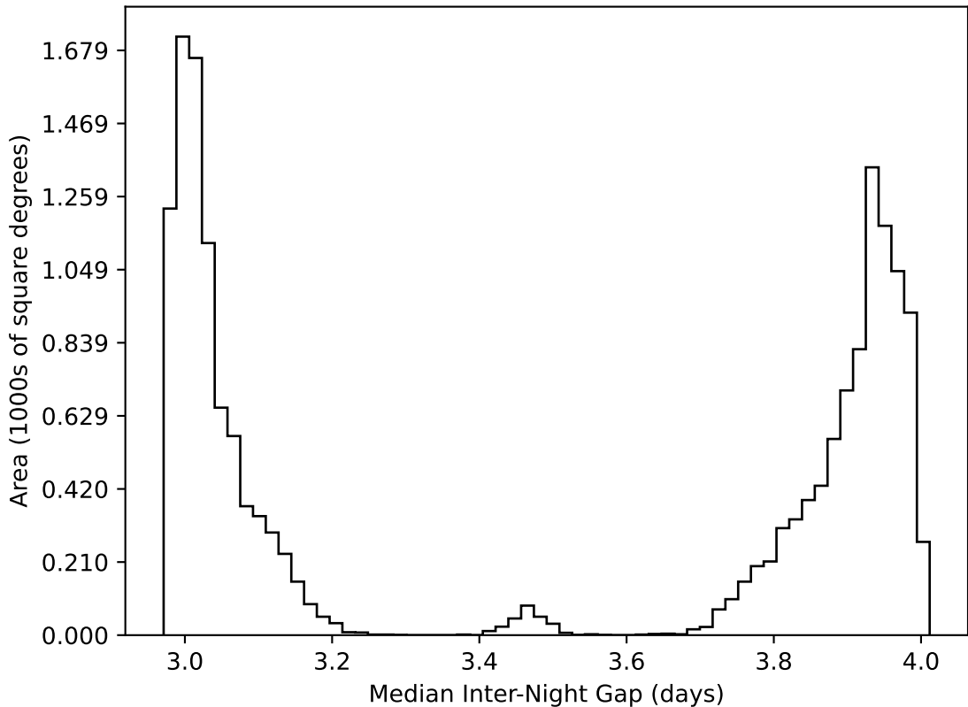
noroll_mjdp180_v3.4_10yrs WFD all bands: Median Inter-Night Gap
