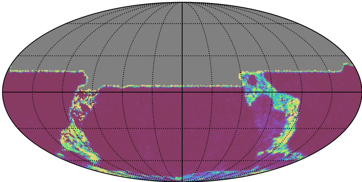
noroll_mjdp180_v3.4_10yrs All sky u band: Median Inter-Night Gap
