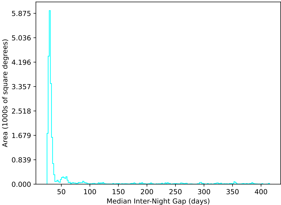
noroll_mjdp180_v3.4_10yrs All sky u band: Median Inter-Night Gap
