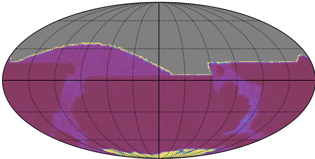
noroll_mjdp180_v3.4_10yrs All sky r band: Median Inter-Night Gap
